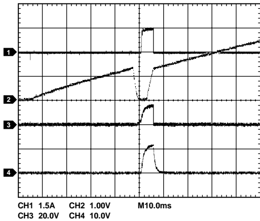
Figure 42. Overcurrent Condition at Startup (ADM1175-1 Model) (CH1 = I_{LOAD} , CH2 = V_{TIMER} , CH3 = V_{GATE} , CH4 = V_{OUT} )
