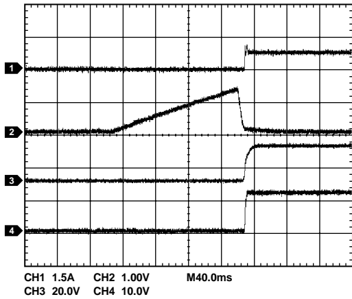
Figure 41. Inrush Current Control into 220 \mu F Load (CH1 = I_{LOAD} , CH2 = V_{TIMER} , CH3 = V_{GATE} , CH4 = V_{OUT} )
