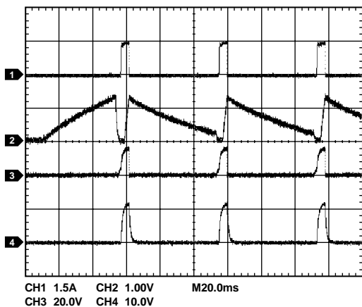
Figure 43. Overcurrent Condition at Startup (ADM1175-2 Model) (CH1 = I_{LOAD} , CH2 = V_{TIMER} , CH3 = V_{GATE} , CH4 = V_{OUT} )
