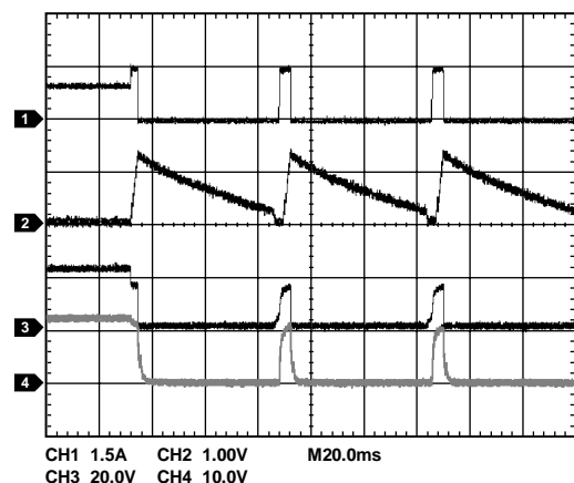
Figure 45. Overcurrent Condition During Operation (ADM1175-2 Model) (CH1 = I_{LOAD} , CH2 = V_{TIMER} , CH3 = V_{GATE} , CH4 = V_{OUT} )
