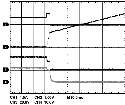
Figure 44. Overcurrent Condition During Operation (ADM1175-1 Model) (CH1 = I_{LOAD} , CH2 = V_{TIMER} , CH3 = V_{GATE} , CH4 = V_{OUT} )
