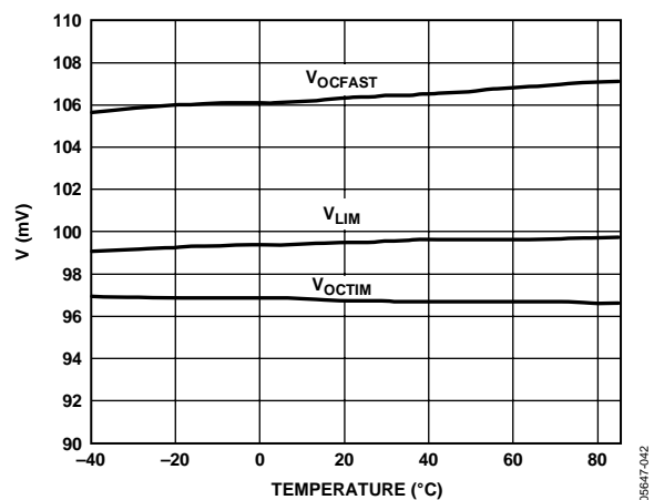
Figure 23. V_{OCTIM} , V_{LIM} , V_{OCFAST} vs. Temperature
