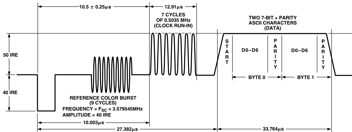
Figure 95. Closed Captioning Waveform (NTSC)
