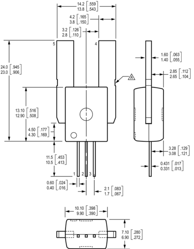
Package CB-PSS
