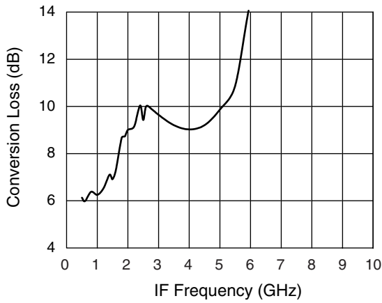
Performance vs. IF Frequency F_{RF} = 38 \text{ GHz} , F_{LO} = F_{RF} - F_{IF} , P_{LO} = 9 \text{ dBm}
