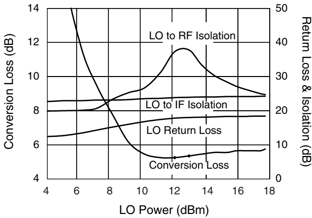
Performance vs. LO Power F_{RF} = 38 \text{ GHz} , F_{LO} = 37 \text{ GHz} , P_{RF} = -10 \text{ dBm}
