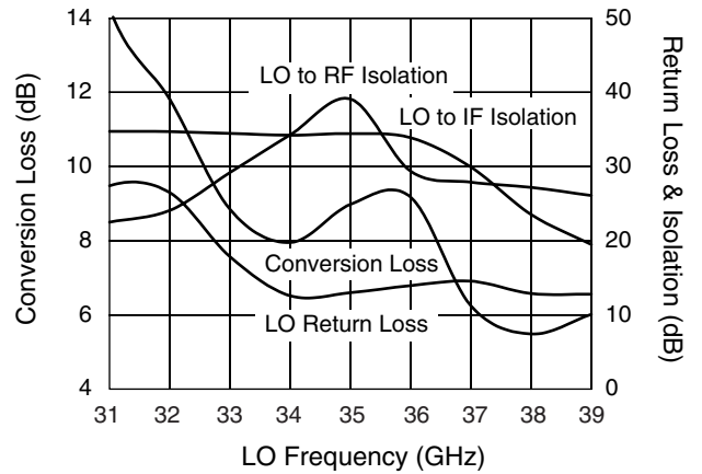
Performance vs. LO Frequency F_{RF} = F_{LO} + 1 \text{ GHz} , P_{LO} = 9 \text{ dBm}
