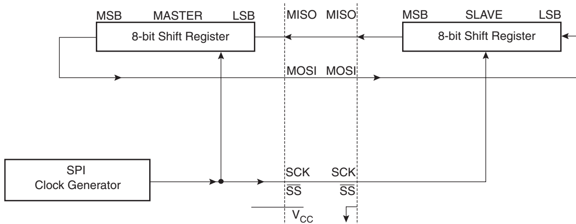
Figure 17. SPI Master/Slave Interconnection
