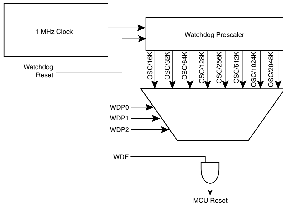
Figure 15. Watchdog Timer
