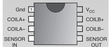
8L PDIP
