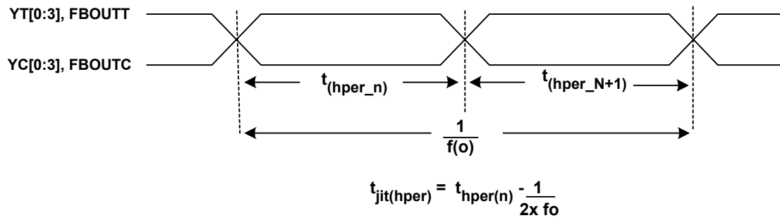
Figure 4. Half-period Jitter
