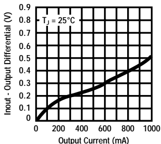
Dropout Voltage
